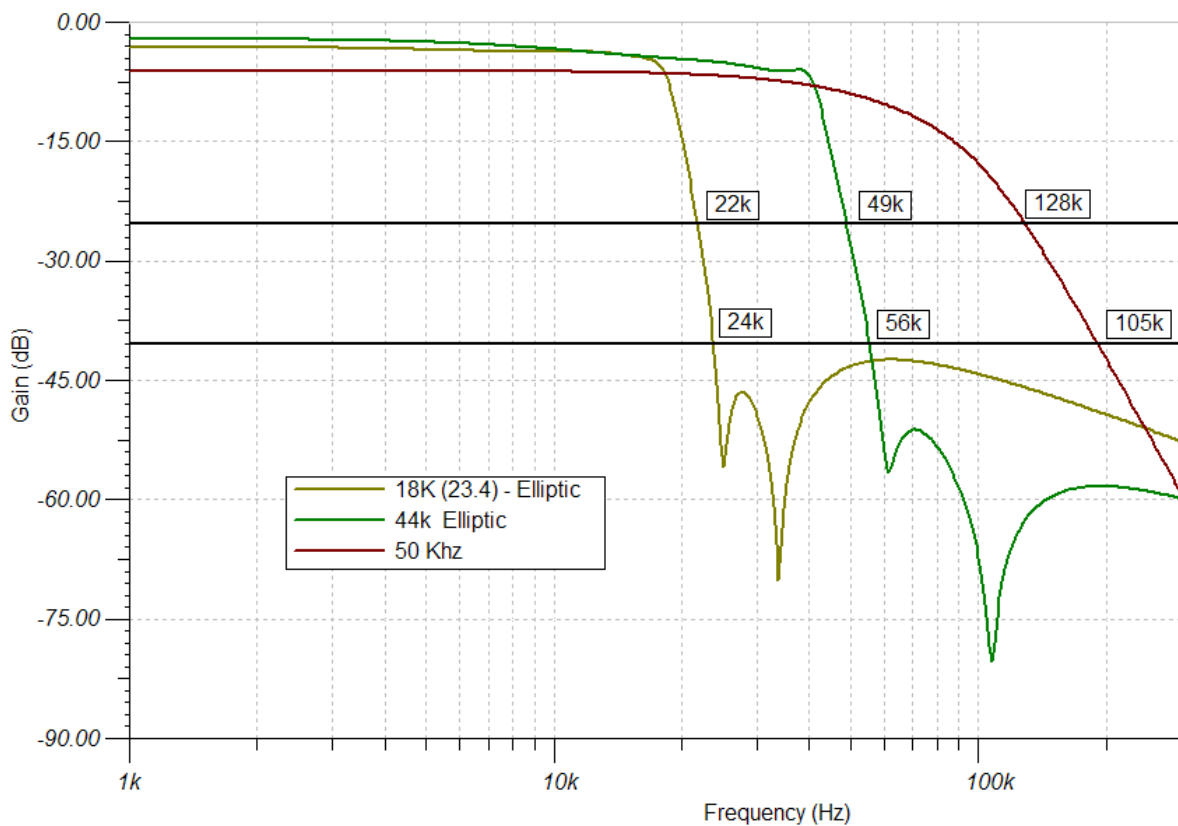
Figure 34: The low pass filters of Pre-Amplifier PCB 14 and Amplifier PCB 13
