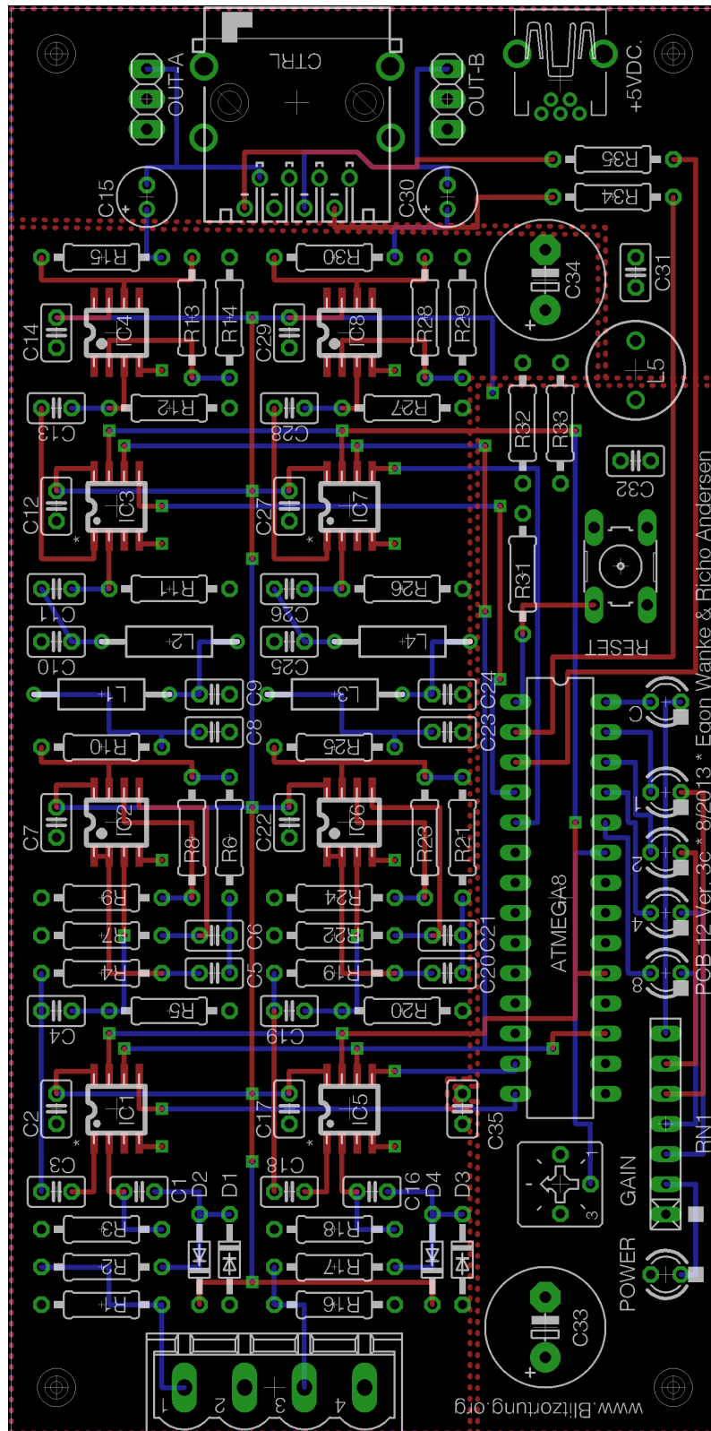
Figure 30: The Printed Circuit Board of Amplifier PCB 12 Version 3
