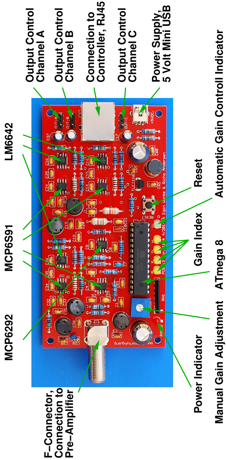
Figure 39: An assembled Amplifier PCB 13 Version 1
