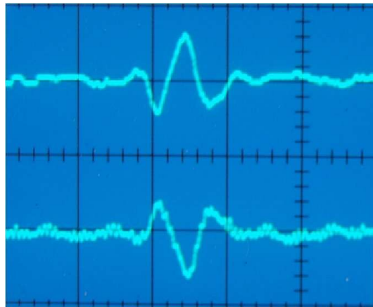
Figure 27: A signal of a lightning discharge received by an electrical antenna (above) and by a ferrite rod antenna (below)
