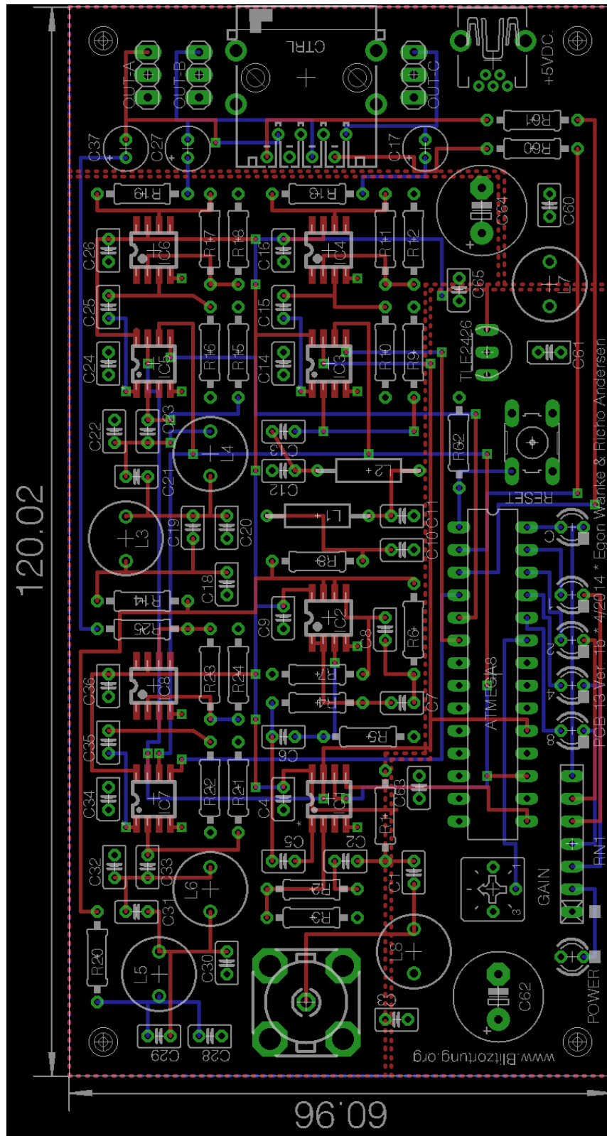
Figure 37: The Printed Circuit Board of Amplifier PCB 13 Version 1
