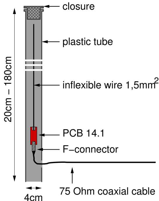
Figure 24: An example of an e-field antenna
