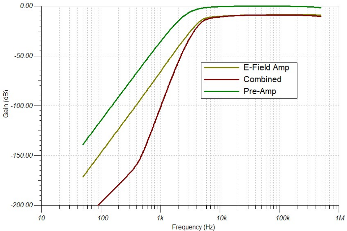
Figure 33: The high pass filters of Pre-Amplifier PCB 14 and Amplifier PCB 13
