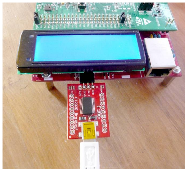
Figure 57: A serial-to-USB adapter connected to the controller
