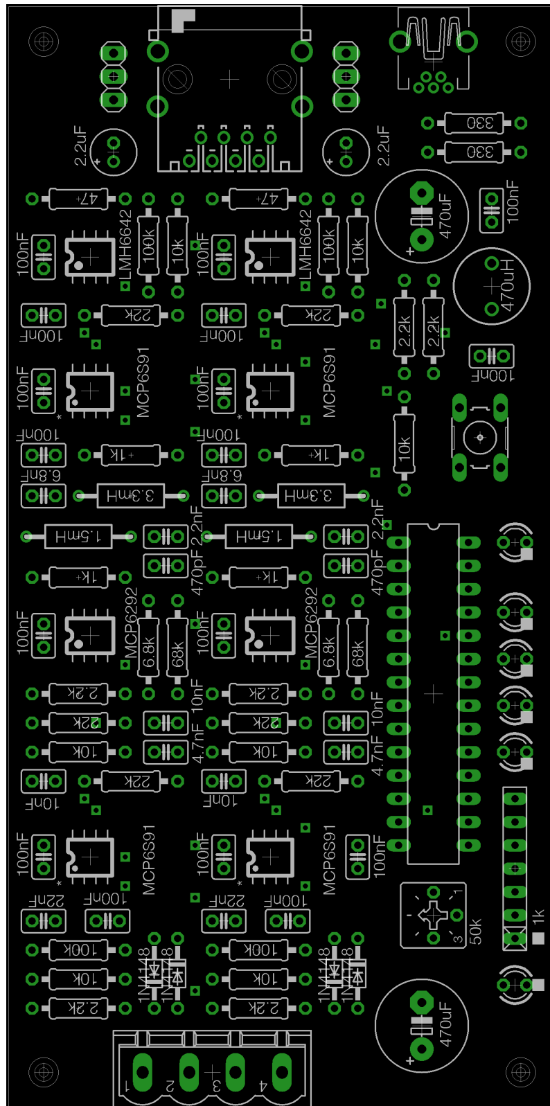
Figure 31: Assembly Diagram of Amplifier PCB 12 Version 3
