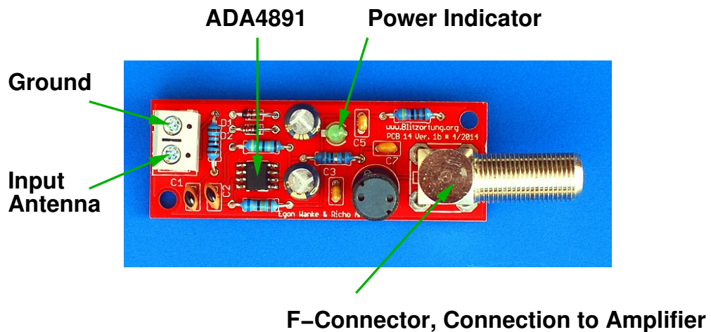
Figure 41: The Printed Circuit Board, the Assembly Diagram, and an assembled Amplifier PCB 14 Version 1
