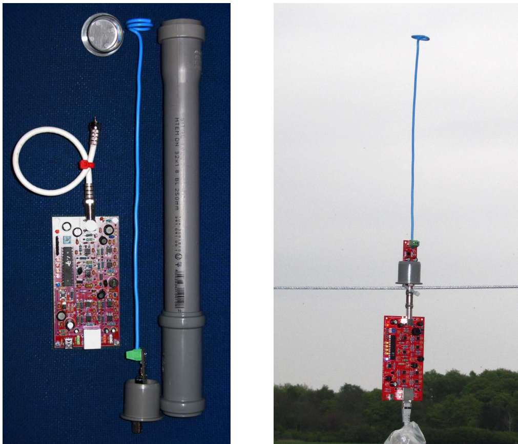
Figure 26: An e-field antenna build with a 30cm wire
