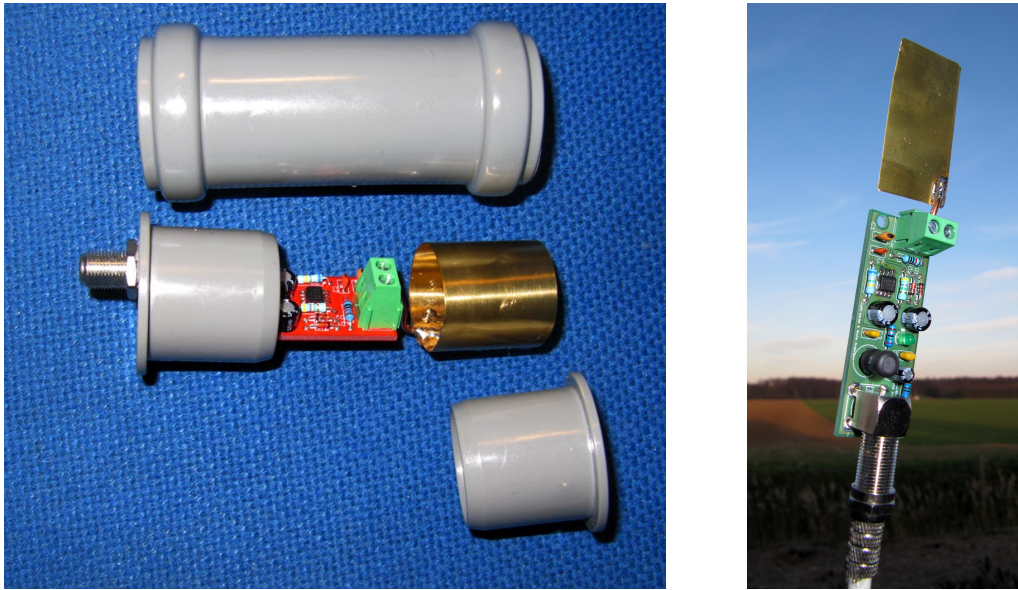
Figure 25: An e-field antenna build with copper plates
