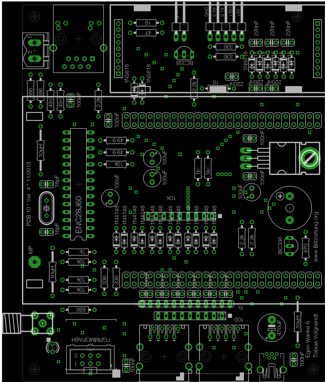
Figure 45: Assembly Diagram of Controller 10.4
