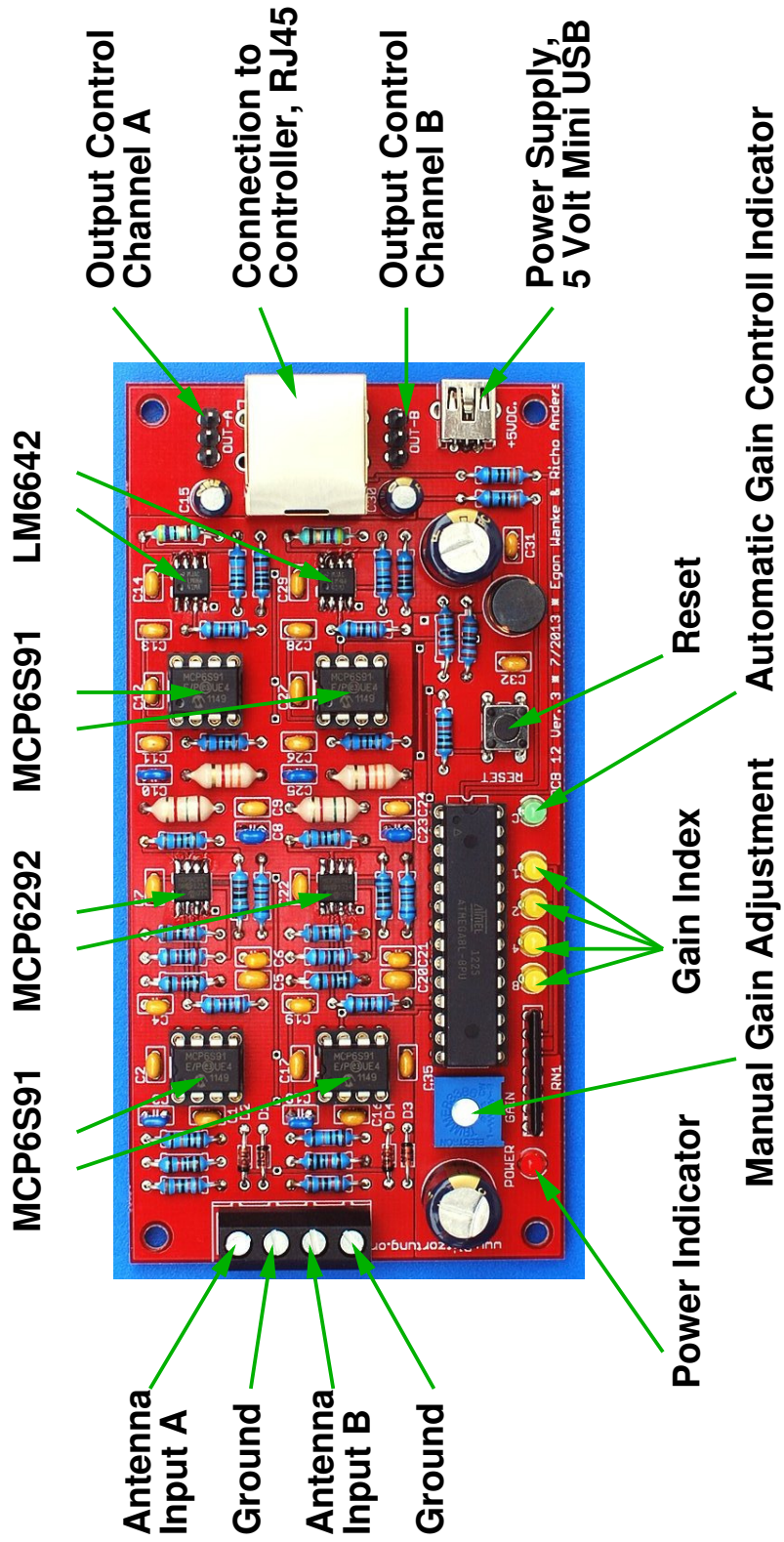
Figure 32: An assembled Amplifier PCB 12 Version 3
