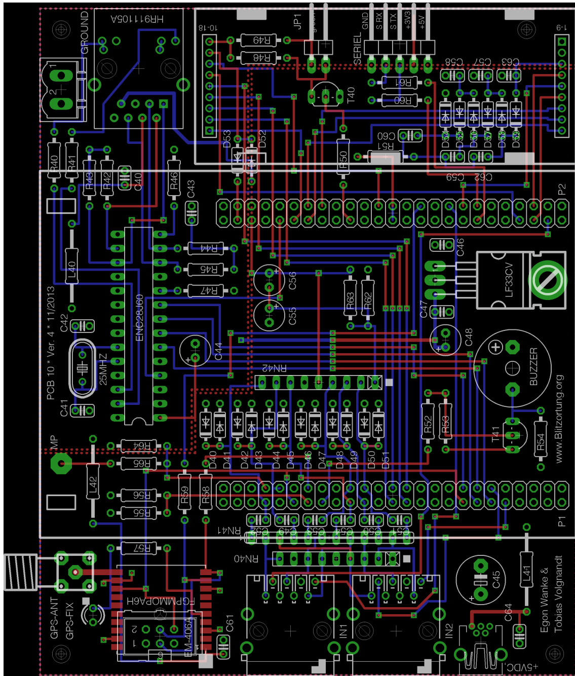
Figure 44: Printed Circuit Board of Controller 10.4
